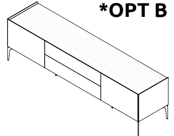
TV206N-2K2F/SKY45 LWH - 2062x470x560
