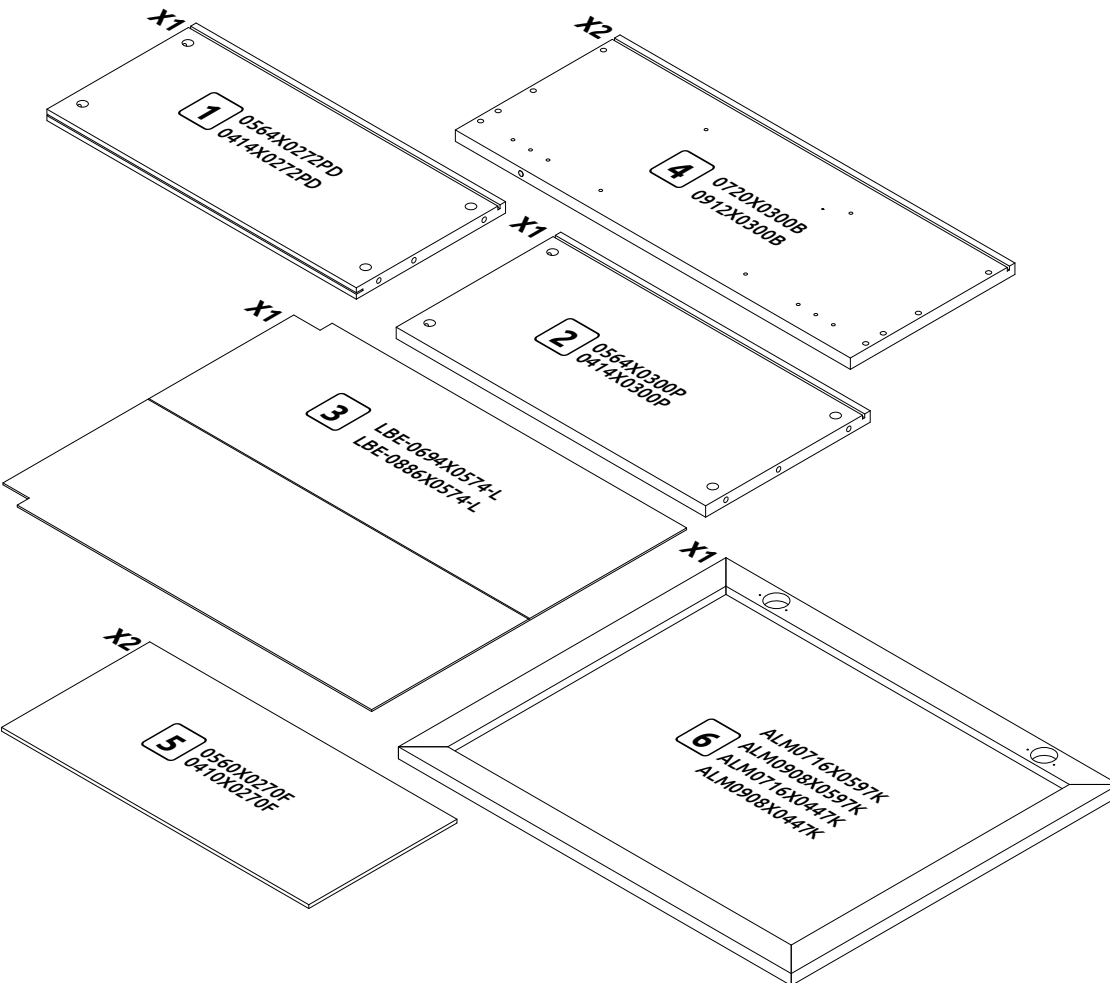
V7-60-1AL LHW-600x720x320
