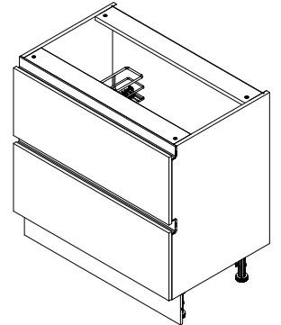
R-90-2MZ LHW-900X943X600
