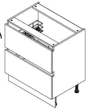
R-80-2MZ LHW-800X943X600
