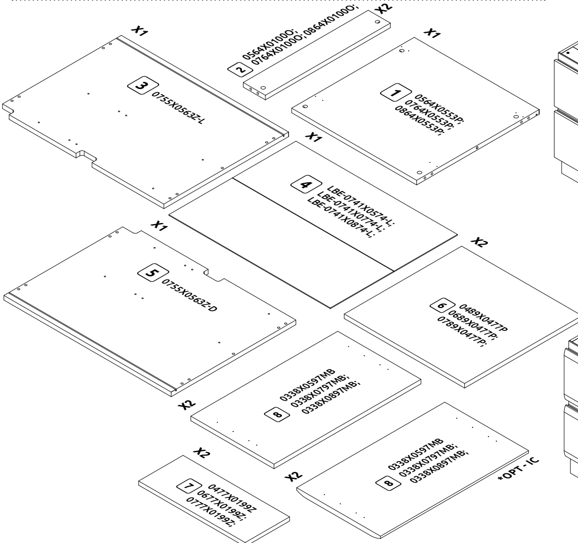
R-90-2MBOX LHW-900X943X600
