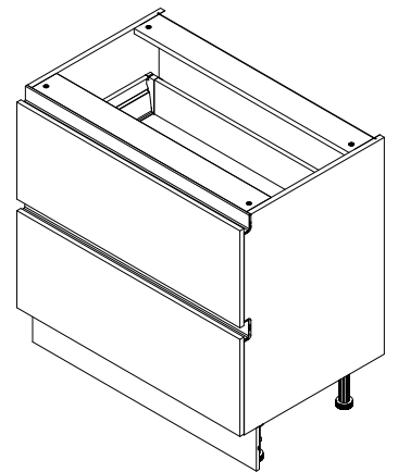
R-90-2MBOX LHW-900X943X600
