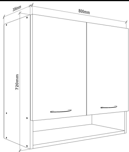
Gornji element V80P2
