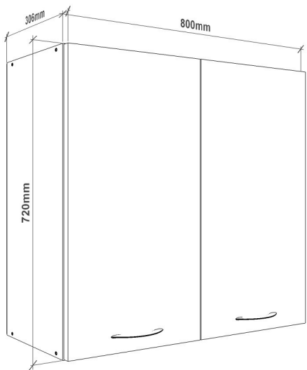
Gornji element V80
