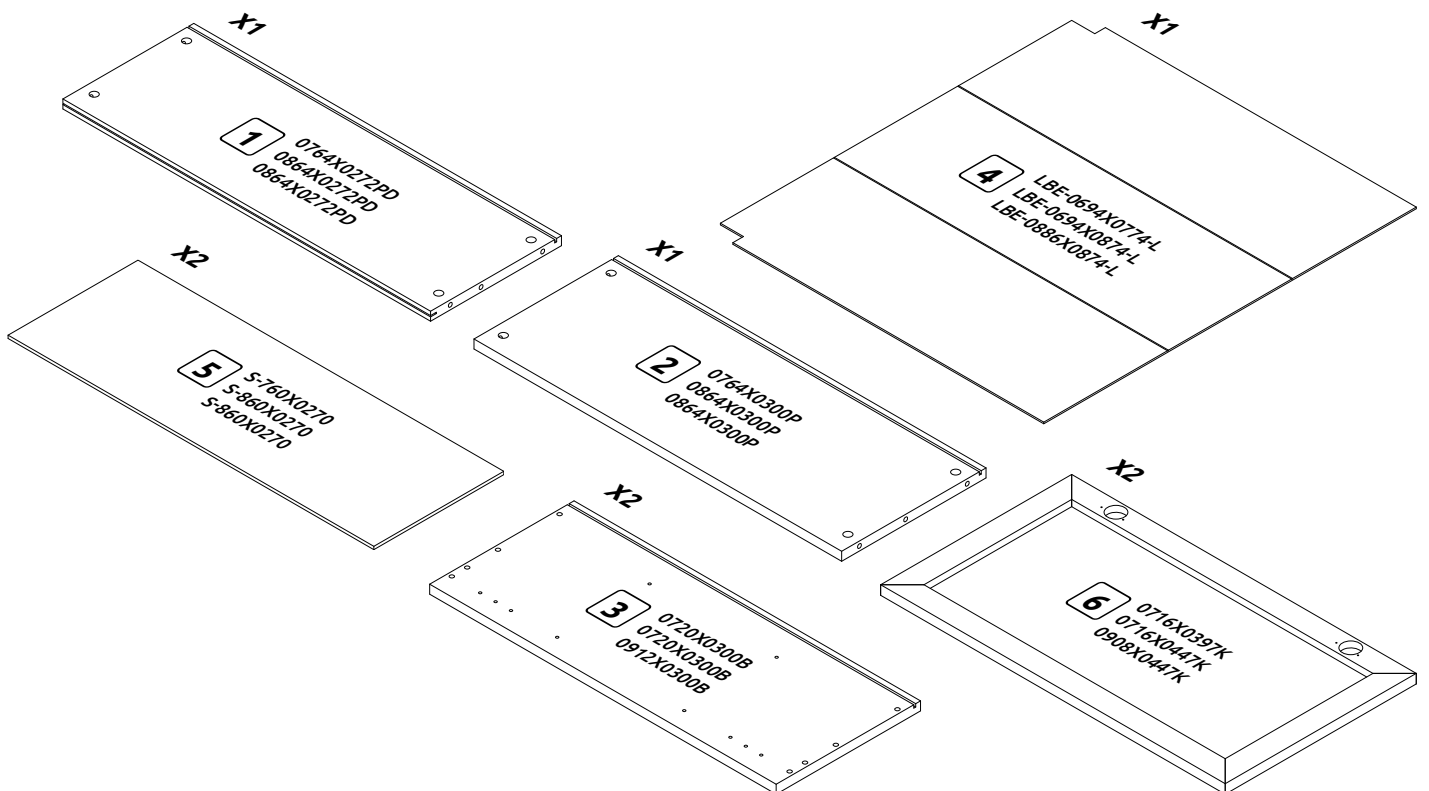
V7-80-2AL LHW-800x720x320
