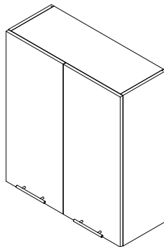
V9-80-2K 800x912x320
