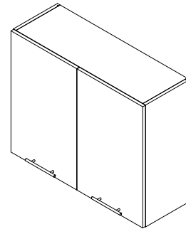
V7-90-2K 900x720x320
