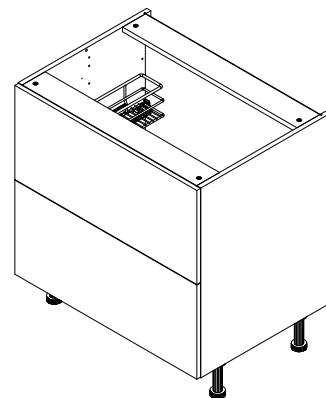
R-80-2MZ LWH - 800x870x600
