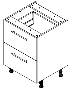
R-60-2MBOX LHW-600X870X600
