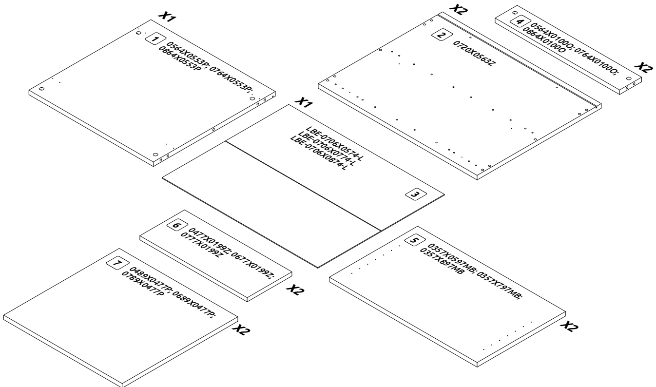
R-90-2MBOX LHW-900X870X600
