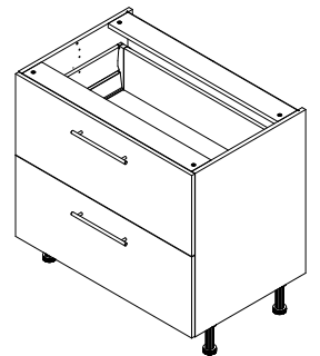
R-90-2MBOX LHW-900X870X600
