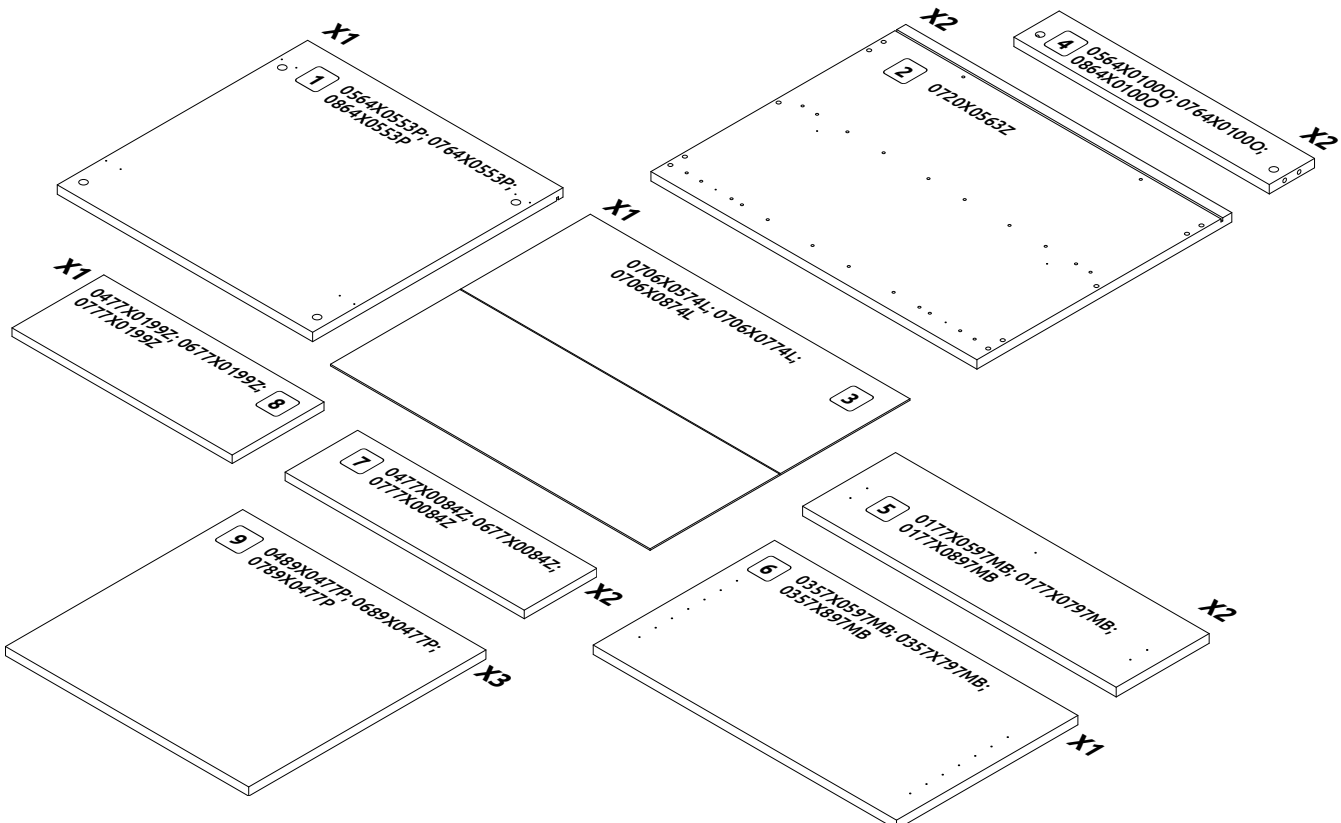
R-90-3MBOX LHW-900X870X600
